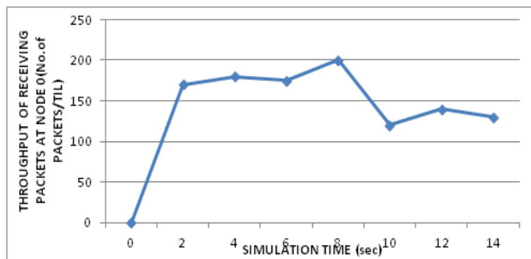
Fig. 1 Simulation time vs Throughput of receiving packets
