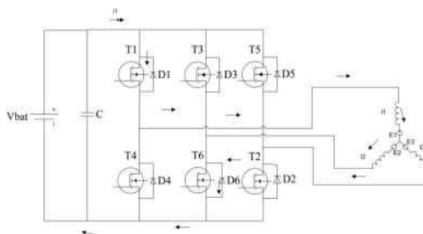
Figure: motoring mode
