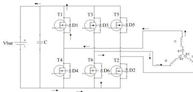
Figure: regenerative mode
