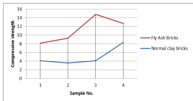
Fig. 1: Fly Ash Bricks Vs Clay Bricks-A
