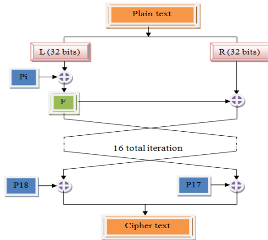
Fig 8: Blowfish encryption algorithm
