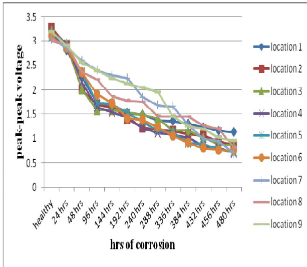
(a) Trends of peak-peak voltage for location 1-9
