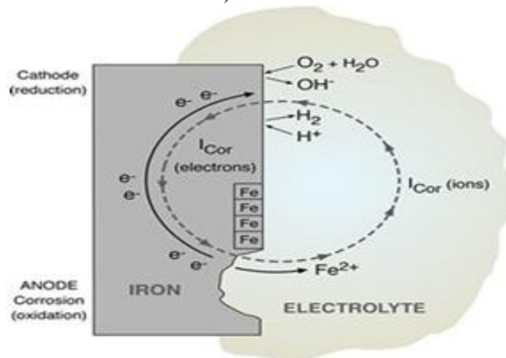
Figure1: Mechanism of Corrosion
