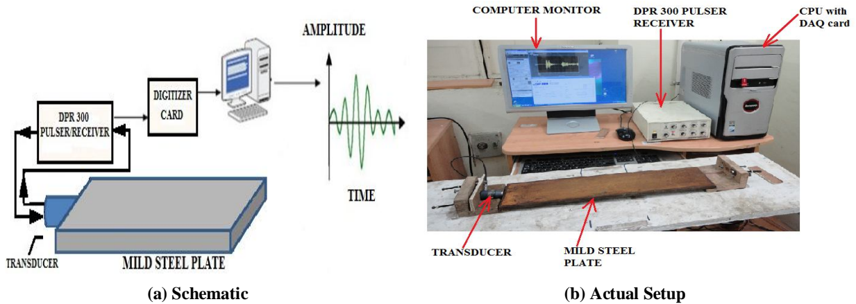
Fig. 5: Ultrasonic Investigations for capturing the wave signatures
