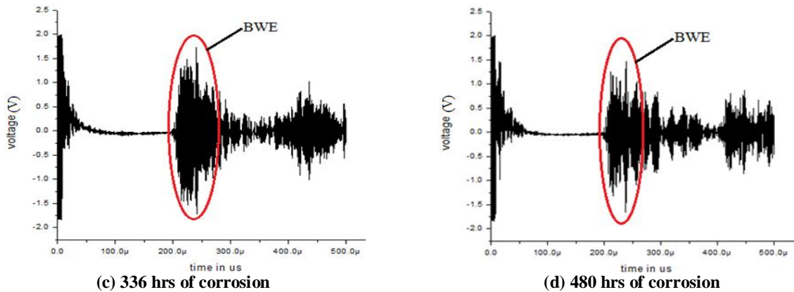
Fig.7: Signatures of 0.5MHz frequency at location 11
