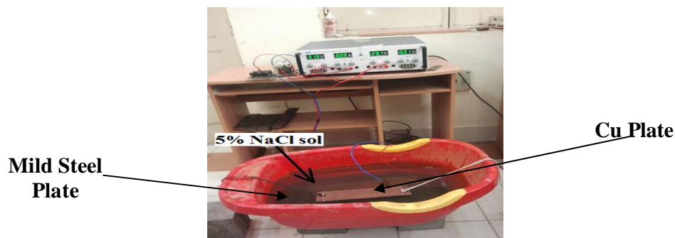
Figure 3: Setup for impressed current corrosion
