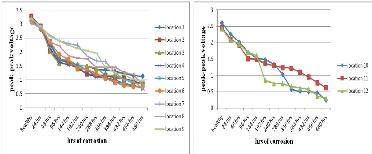
(a) Trends of peak-peak voltage for location 1-9
