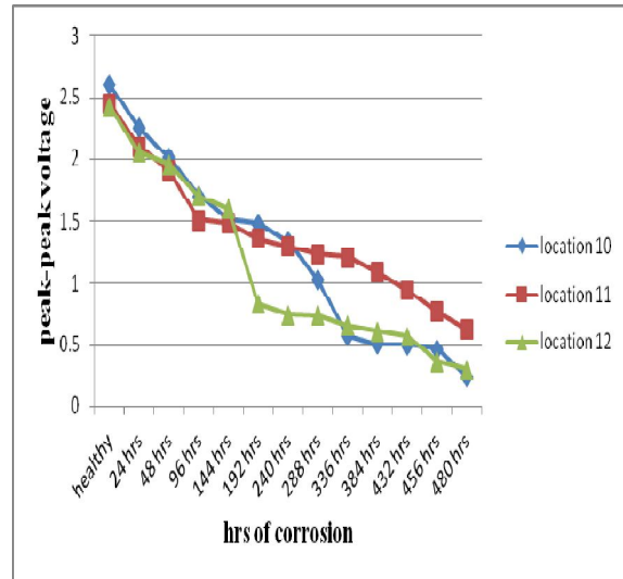
(b) Trends of peak-peak voltage for location 10-12
