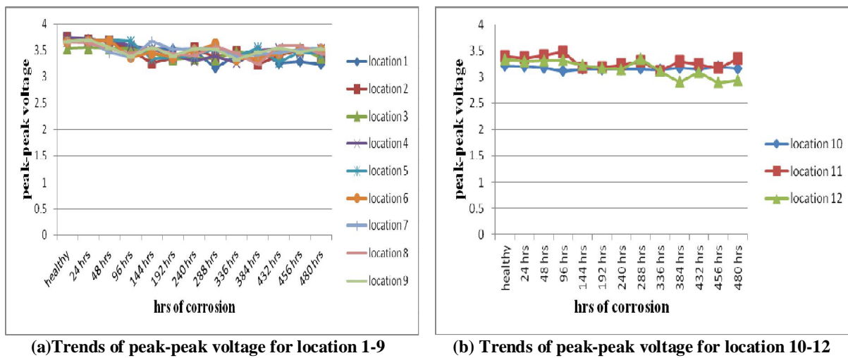
Fig.8: Results of 0.5MHz frequency
