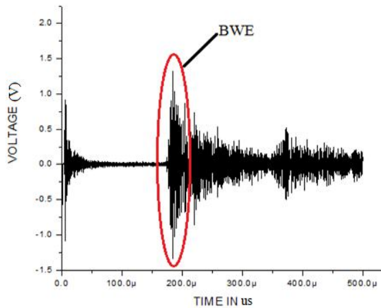
(a) Healthy signatures
