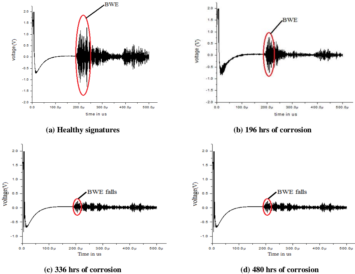
Fig.9: Signatures of 1MHz frequency at location 11
