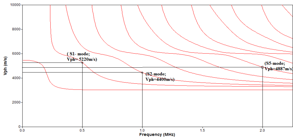
Fig. 7: Dispersion curves for Lamb wave propagation in a 12 mm steel plate in air
