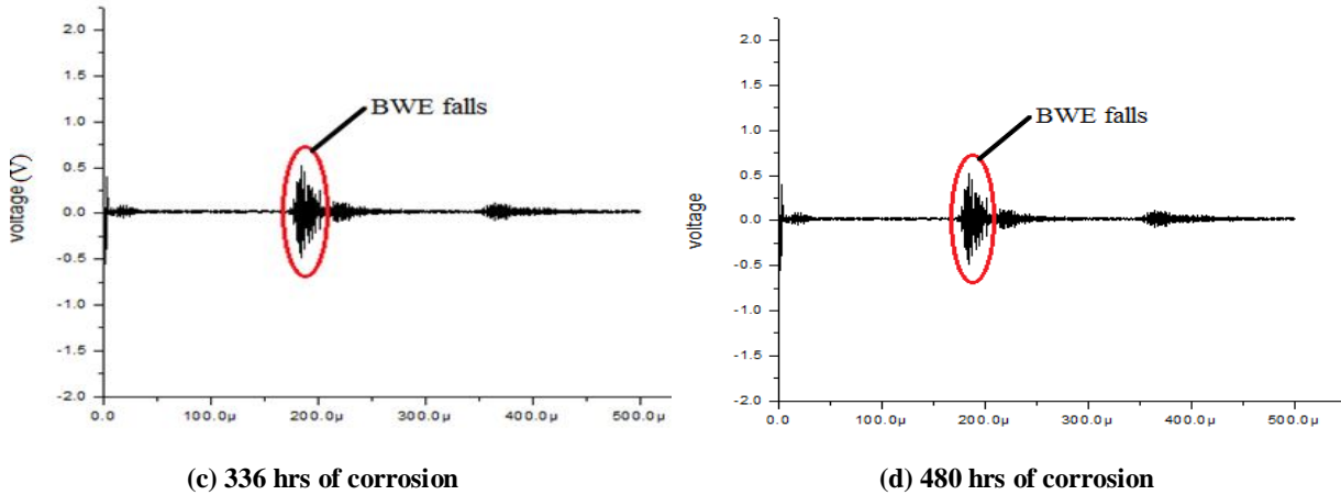
Fig.11: Signatures of 2MHz frequency at location 11
