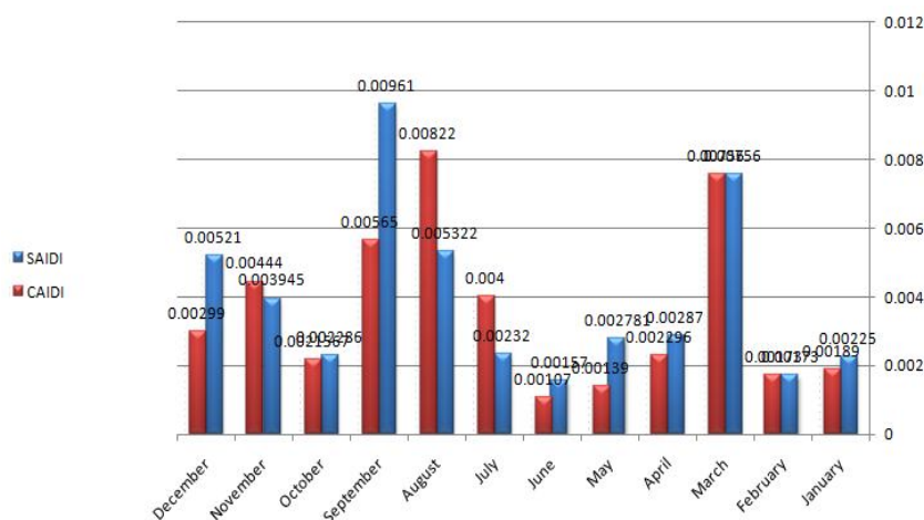
Figure (4):- SAIDI ,CAIDI Sketch shows during the year 2011 to lines 33kv
