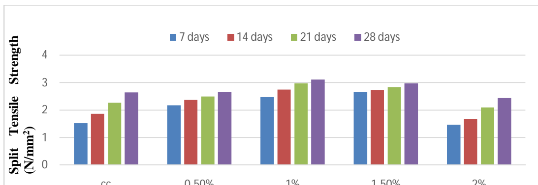
Fig 2. Split Tensile strength of concrete
