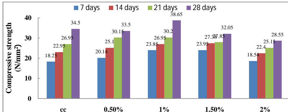
Fig 1. Compressive strength of concrete
