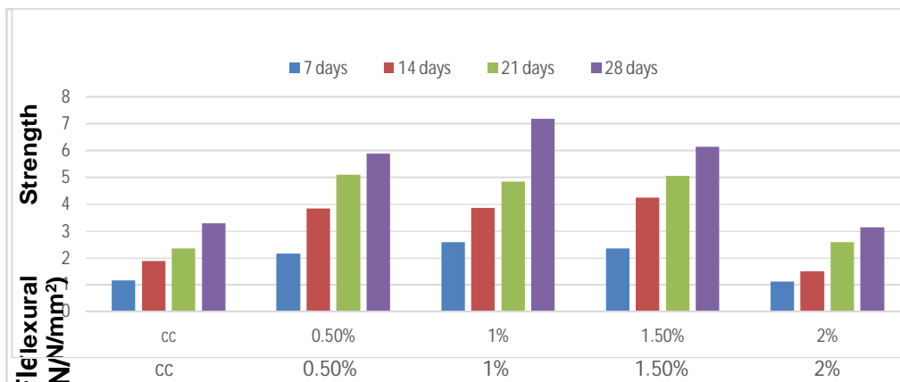
Fig 3. Flexural strength of concrete
