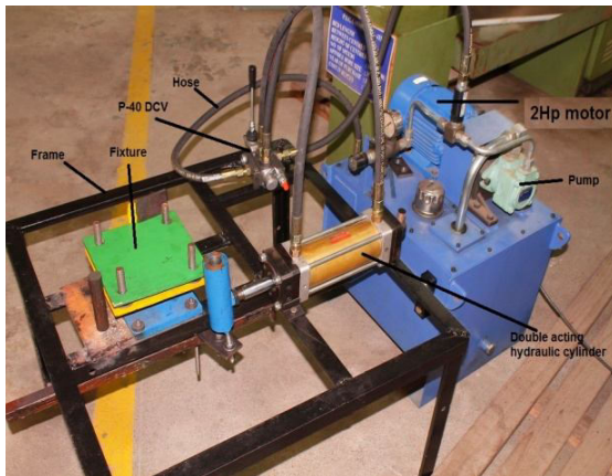
Figure 1.6 Fabricated Model
