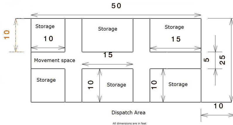
Fig. 7: Optimized Layout of Storage Space
