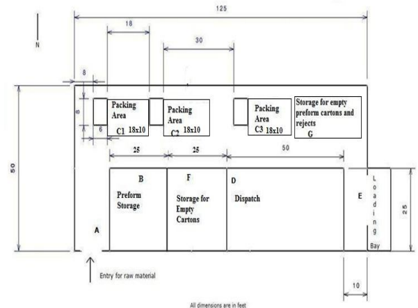
Fig. 6: Final Layout of Unit B
