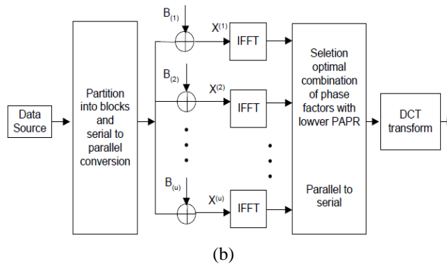
Figure 3: Block Diagram of DCT-SLM scheme
