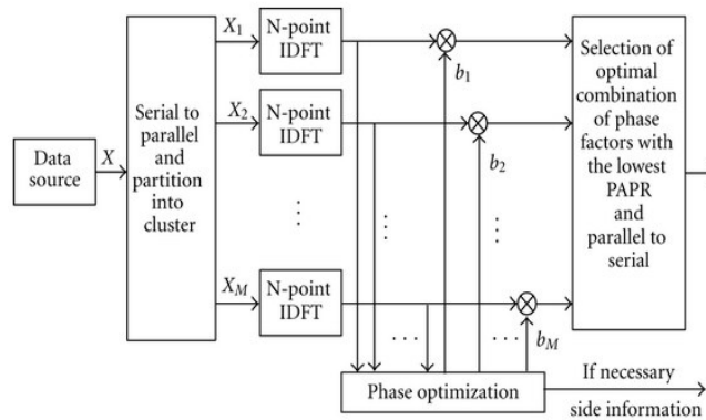
Figure 1: Block diagram of conventional PTS scheme [19].
