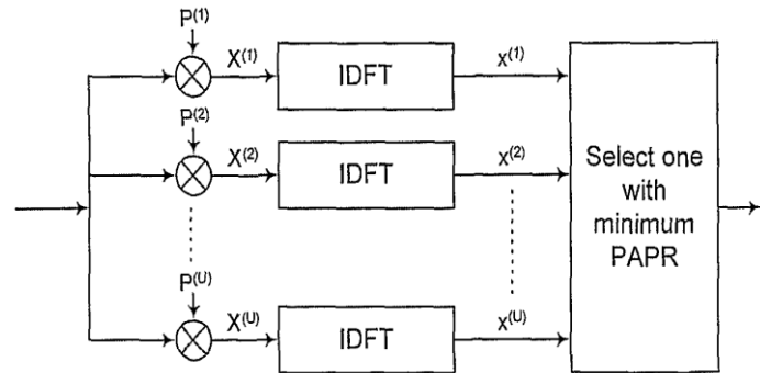
Figure 2: block diagram of SLM technique [20]
