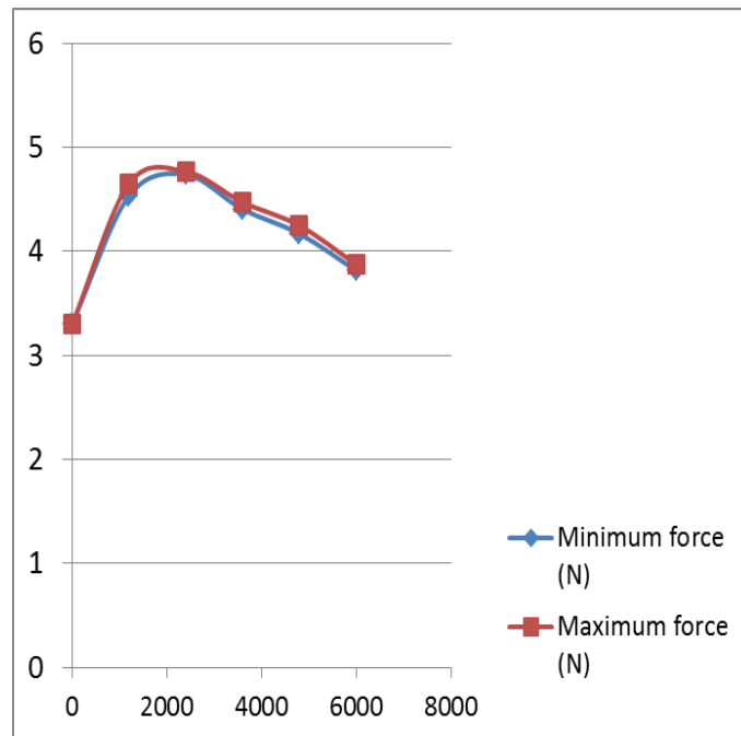
Graph 3) Characteristic curves (force versus speed) for rotating shaft with a constant gap of 4.92 mm.
