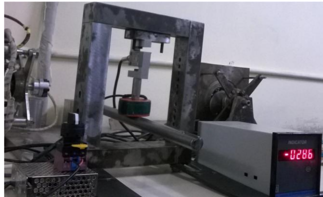
Fig. 6) Gap between the electromagnet and shaft is ZERO with an impulse on shaft at static condition.
