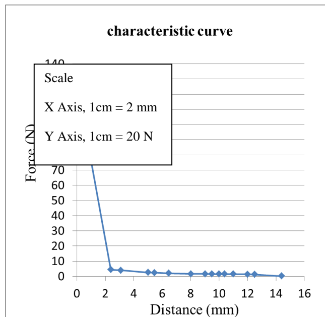
Graph 1) Characteristic curves (force v/s distance) for shaft at static condition
