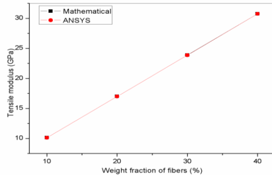
Figure.4 Tensile modulus for 10%, 20%, 30% and 40% addition of E-glass fiber reinforced polyester composites using mathematical and simulation approach
