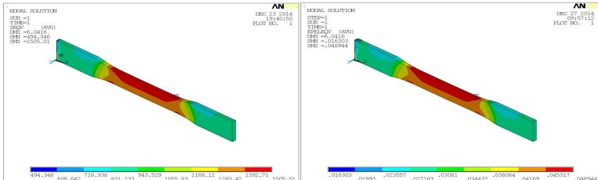
Figure.1 Stress value of E-Glass fiber polyester reinforced composite with 40% weight fraction
