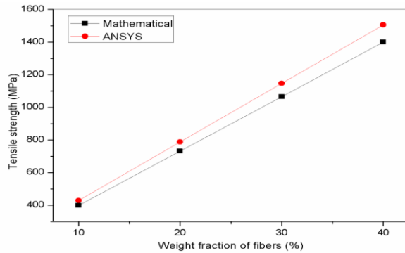
Figure.3 Tensile strength for 10%, 20%, 30% and 40% addition of E-glass fiber reinforced polyester composites using mathematical and simulation approach
