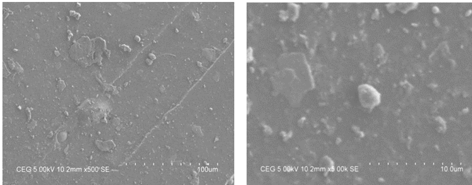
Fig .9 SEM Images of Rubber with 20% Flyash
