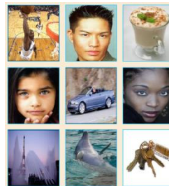
Fig5.2 Story Scheme
