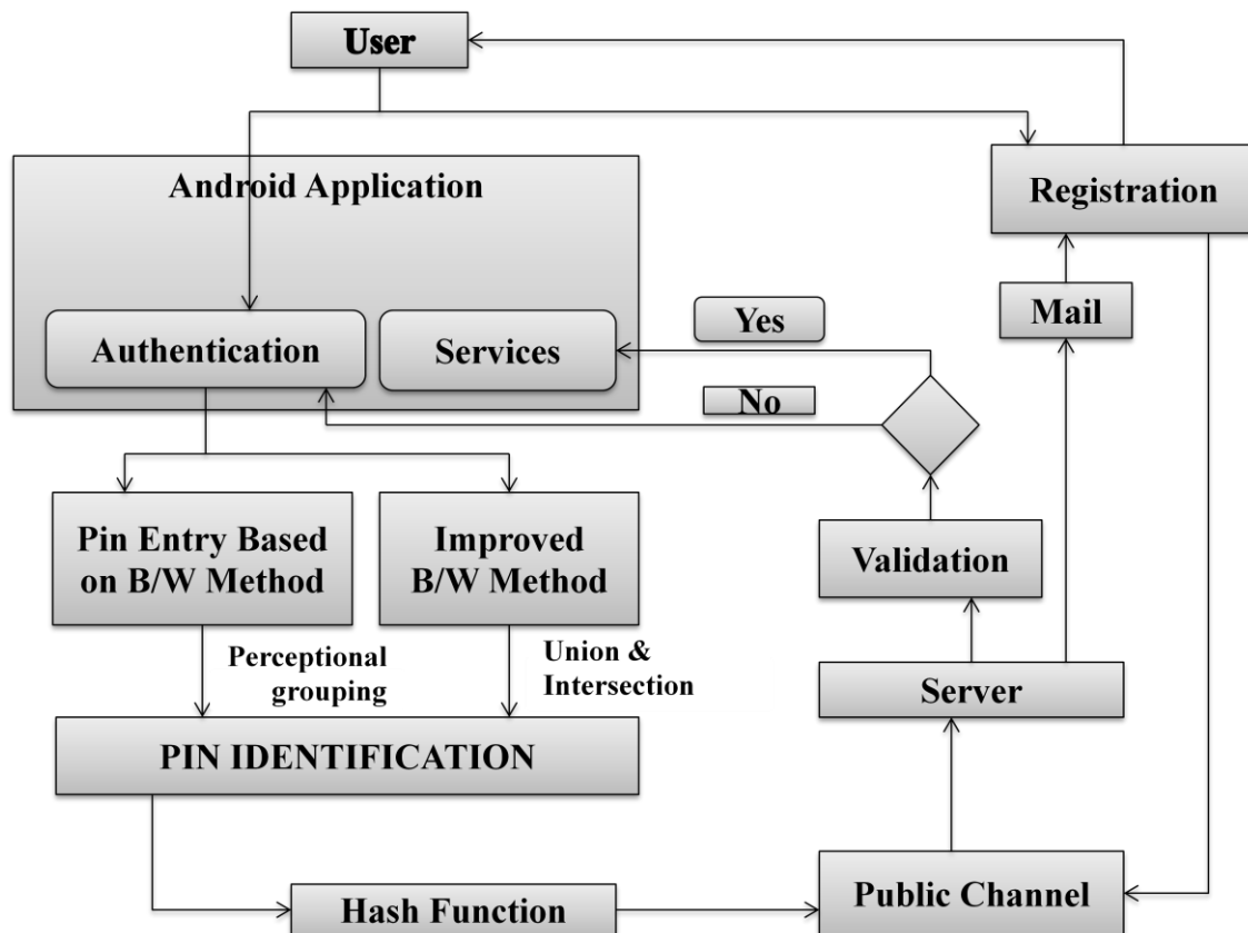
Fig8. Architecture Diagram
