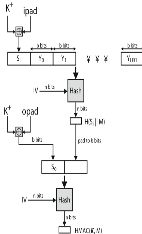
Fig7. HMAC overview
