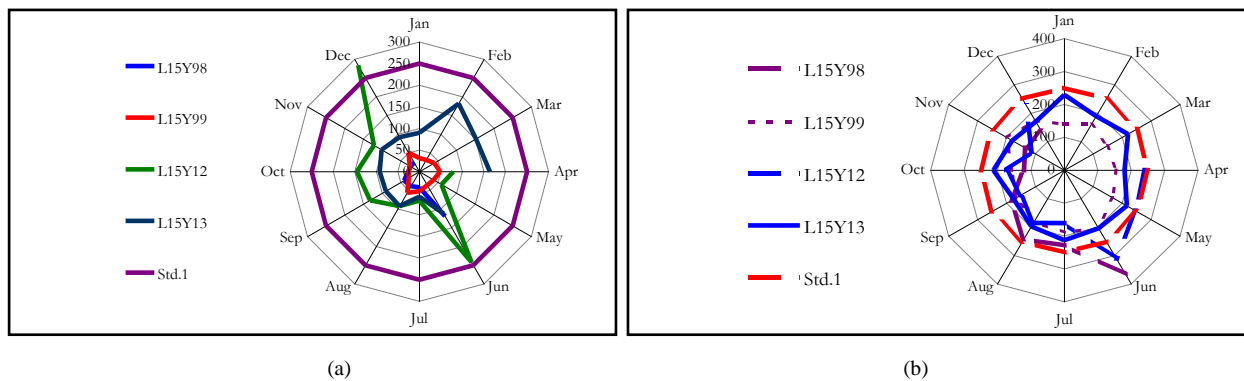
Fig.1.16: L15 during 1998-1999, 2012 – 2013 of (a) COD (b) Chloride.
