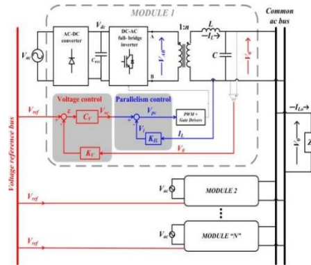
Fig 3. Circuit of VSIs modules connected in parallel
