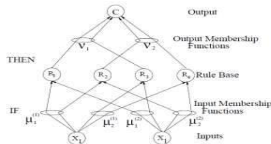
Fig 2. Architecture of four rule fuzzy controller from neural networks point of view. The X-, R-, and C-modules can be viewed as the neurons in a layered neural network and the n-units as the adaptable weights of the network. The X-module layer can easily be identified as the input layer of a multi-input neural network whereas the C-module layer can be seen as the output layer. The R-module layer serves as the hidden or intermediate layer that constitutes the internal representation of the network. The fact that one n-module can be connected to more than one R-module is equivalent to the connections in a neural network that share a common weight. This is of key importance for keeping the structural integrity of the fuzzy controller intact.
