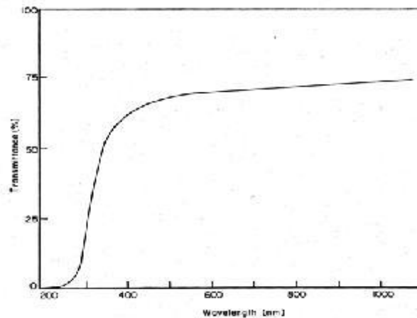
Figure 4. UV-vis – NIR spectrum of GG
