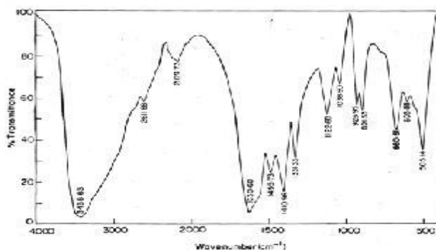
Figure 3. FTIR spectral pattern of GG
