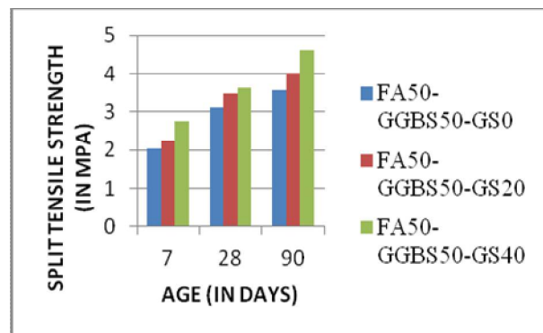
Figure 2. Split Tensile Strength versus age
