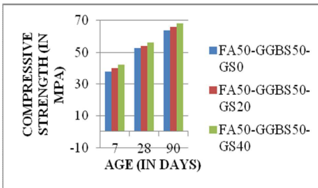
Figure 1. Compressive strength versus age
