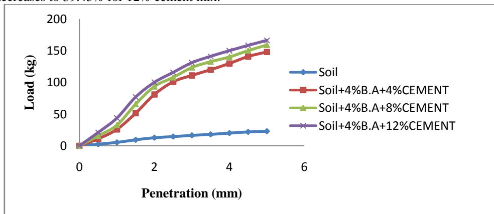
Fig 7: CBR curves of Soil stabilized with 4%ash and varying percentages of cement
