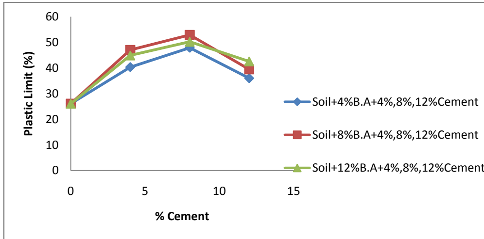
Fig 6: Plastic limit of Soil stabilized with different percentages of Bagasse ash and Cement
