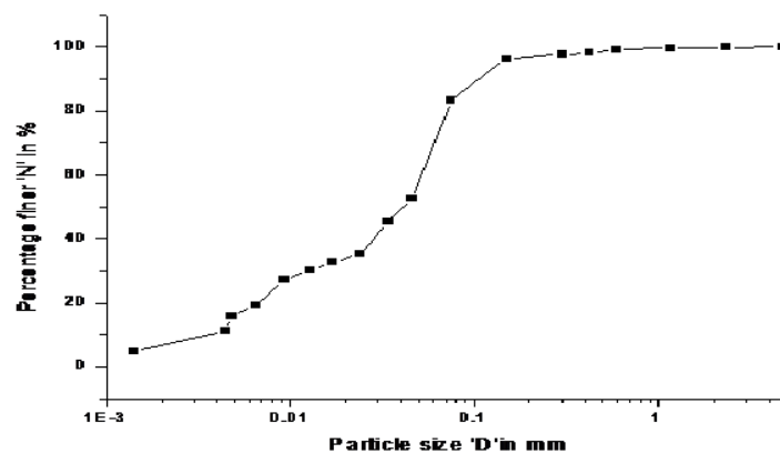
Fig1: Particla Size Distribution curve
