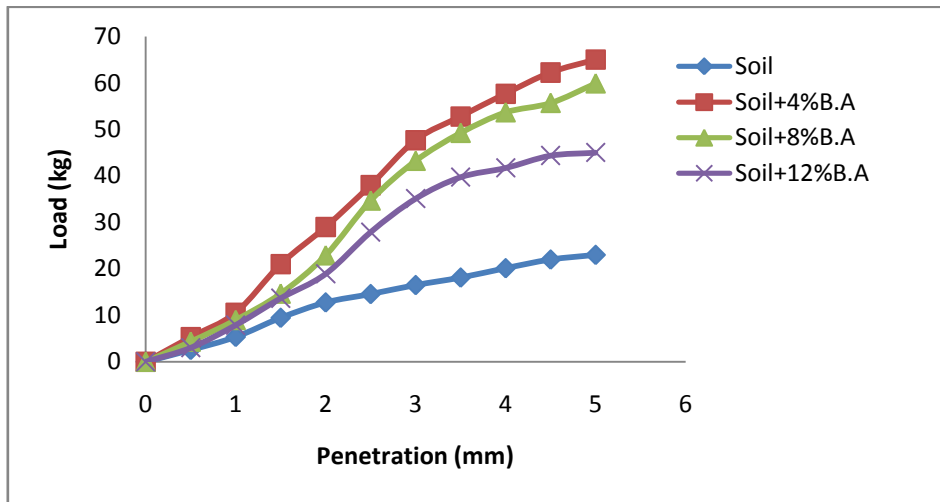
Fig 4: Soaked CBR curves of Soil stabilized with varying percentage of Bagasse ash
