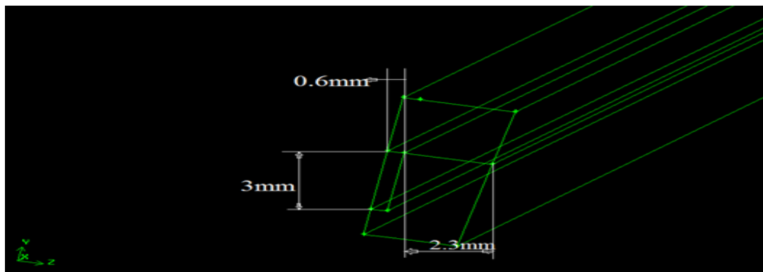
Fig. 1. Channel dimensions.
