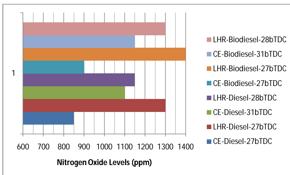
Fig.9 Bar charts showing the variation of nitrogen oxide (NO x ) levels at full load operation with test fuels with conventional engine (CE) and engine with LHR combustion chamber at recommended and optimized injection timings at an injector opening pressure of 190 bar.
