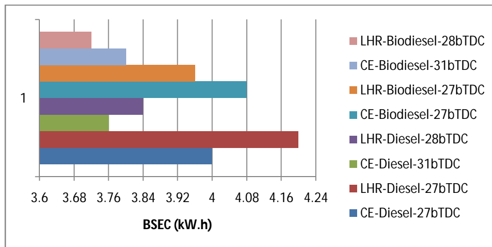
Fig.4.Bar charts showing the variation of brake specific energy consumption (BSEC) at full load operation with test fuels with both versions of the engine at recommended and optimized injection timings at an injector opening pressure of 190 bar.
