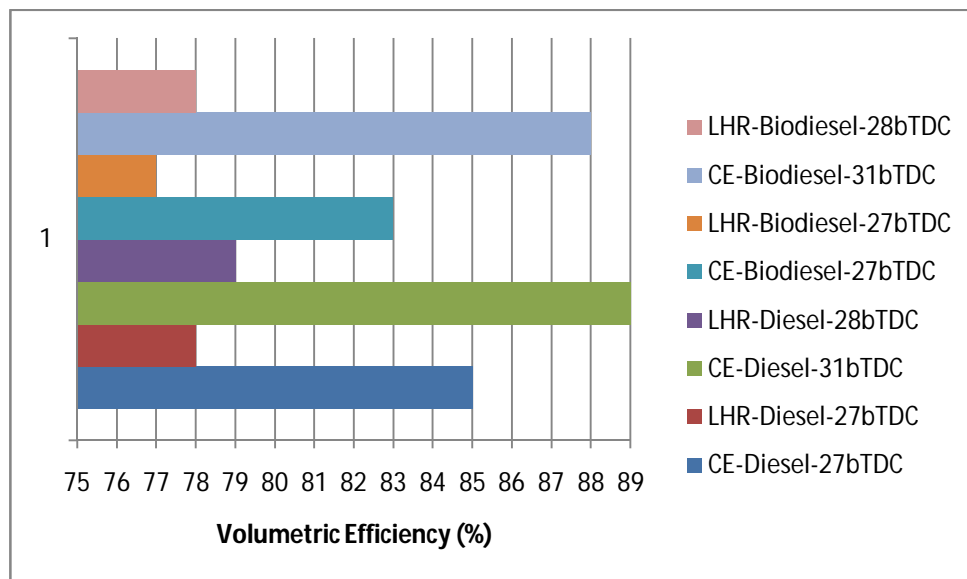
Fig.7 Bar charts showing the variation of volumetric efficiency at full load operation with test fuels with both versions of the engine at recommended and optimized injection timings at an injector opening pressure of 190 bar.
