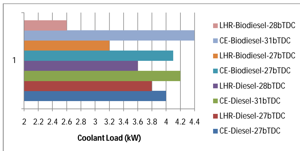
Fig.6 Bar charts showing the variation of coolant load at full load operation with test fuels with both versions of the engine at recommended and optimized injection timings at an injector opening pressure of 190 bar.
