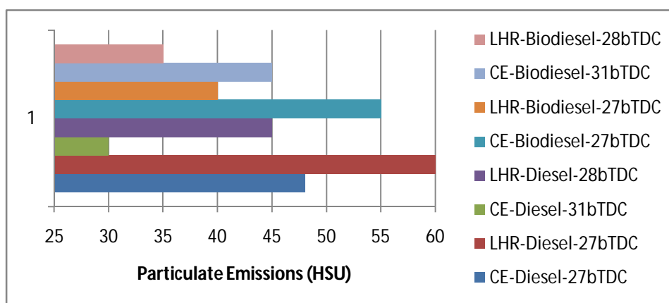
Fig.8. Bar charts showing the variation of particulate emissions at full load operation with test fuels with conventional engine (CE) and engine with LHR combustion chamber at recommended and optimized injection timings at an injector opening pressure of 190 bar.
