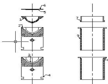
1.Pistoncrown with threads, 2. Superni gasket, 3.Air gap in piston, 4. Body of piston, 5. Ceramic coating on inside portion of cylinder head, 6. Cylinder head, 7.Superni insert with threads, 8.Air gap in liner, 9.Liner
