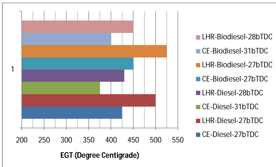
Fig.5 Bar charts showing the variation of exhaust gas temperature (EGT) at full load operation with test fuels with both versions of the engine at recommended and optimized injection timings at an injector opening pressure of 190 bar.
