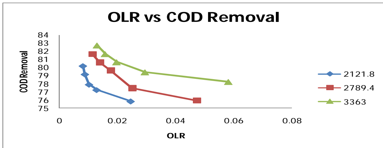
Fig.2 Average Influent COD mg/l Vs varying OLR kg/COD/m 2 day
