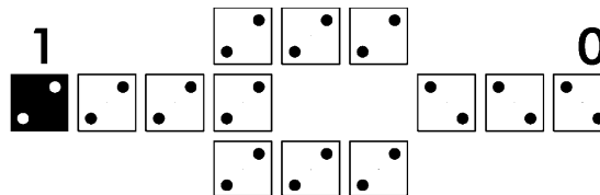
Fig.9 QCA Inverter
