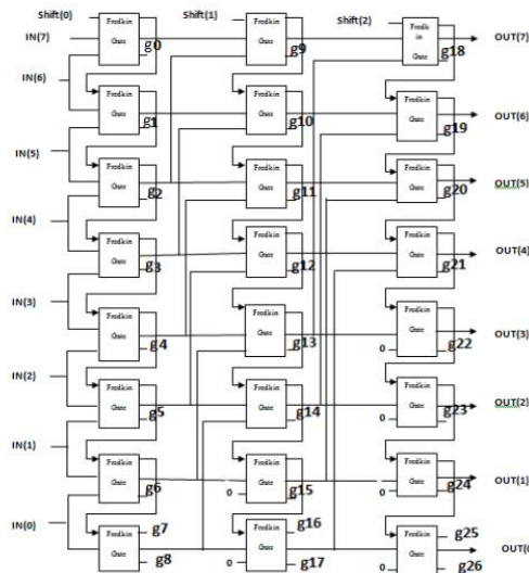
Fig. 11 Barrel Shifter using Fredkin gate
