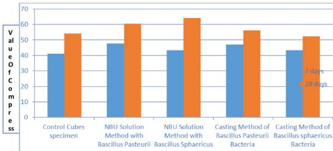
Graph No. 1 Compressive Strength of 7 & 28 Days They are to different Method indicated.
