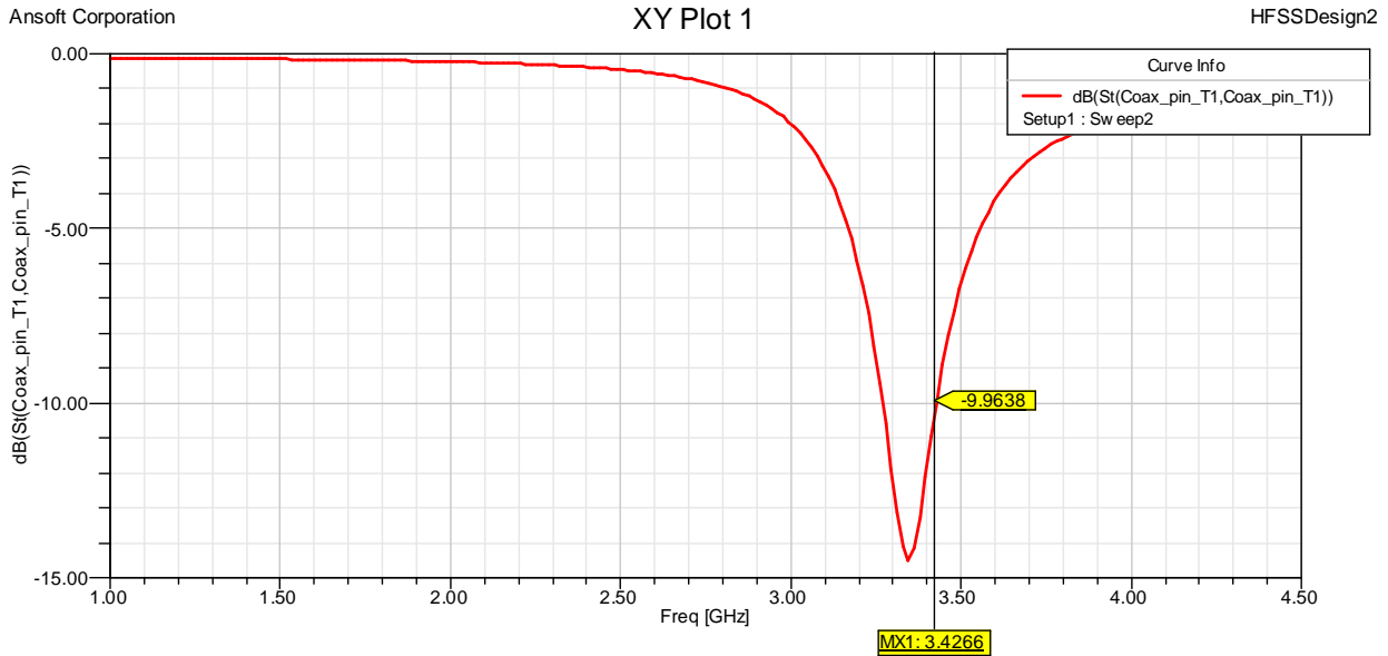
5(b) Rectangular plot of circular patch antenna with partial ground
