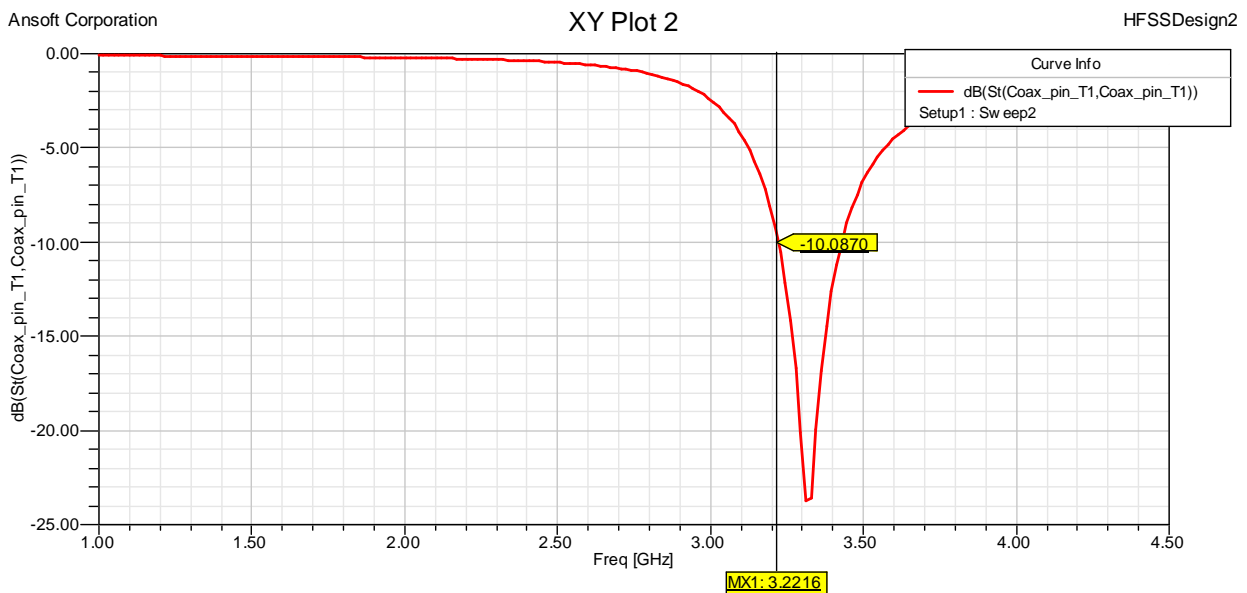
5(c) Rectangular plot of circular patch antenna with partial ground & circular slot.
