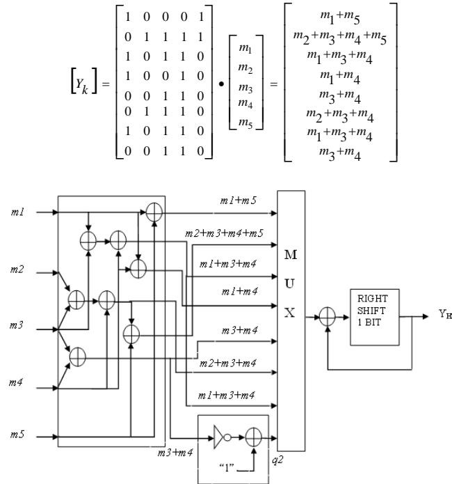
Figure 2: Proposed Architecture 1-D for Low Pass Filter Using NEDA Technique
