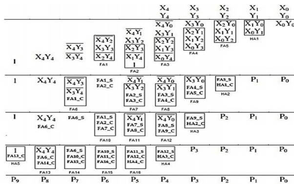
Figure 2: Multiplication by Wallace approach in the circuit
