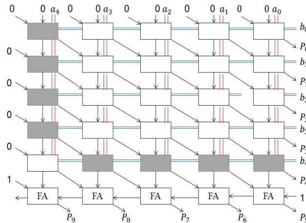
Figure 4: Proposed Design with white and gray cell
