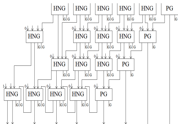
Figure 3: Multi-Operand Addition by Peres and Haghparast-Navi gates
