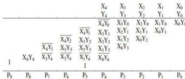
Figure 1: Baugh-Wooley 5 x 5 Signed Multiplier
