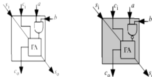
Figure 5: White and gray cell Structure
