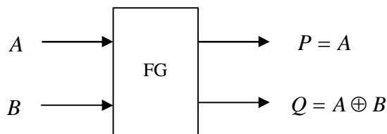
Figure 1: Feynman gate
