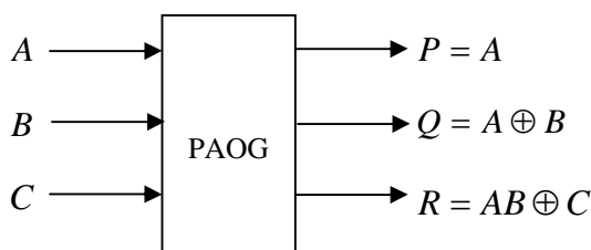
Figure 5: Block Diagram of the PAOG \oplus (AB \oplus C)
