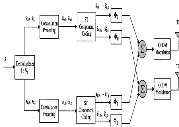
Fig. 2 STF block-coded OFDM with N = 2 and N = 2 .
