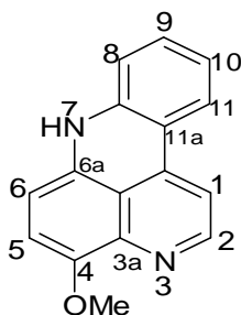
Fig.1:Compound (19)
