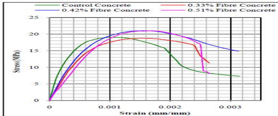
Fig: Average stress-strain curves for prisms with 0, 0.33, 0.42 and 0.51% macro synthetic fiber
