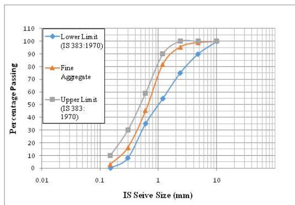
Fig. 3: Grading curve of Fine aggregate
