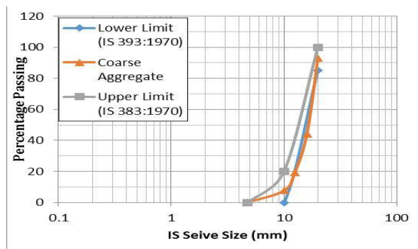
Fig. 1: Grading curve of 20 mm Coarse aggregate
