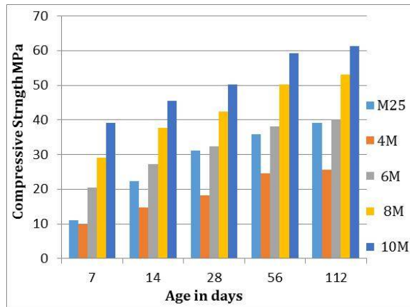
Fig. 6: Compressive strength versus Age
