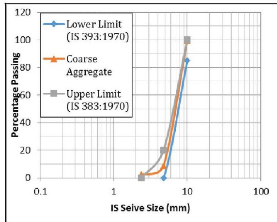
Fig. 2: Grading curve of 10 mm Coarse aggregate
