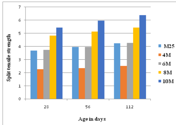
Fig. 7: Split tensile strength of mixes
