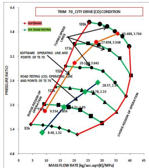
Fig. 7 Turbo match -City Drive - A58N70
