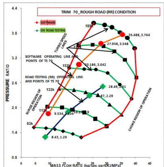
Figure3 Turbo match - Rough Road -A58N70
