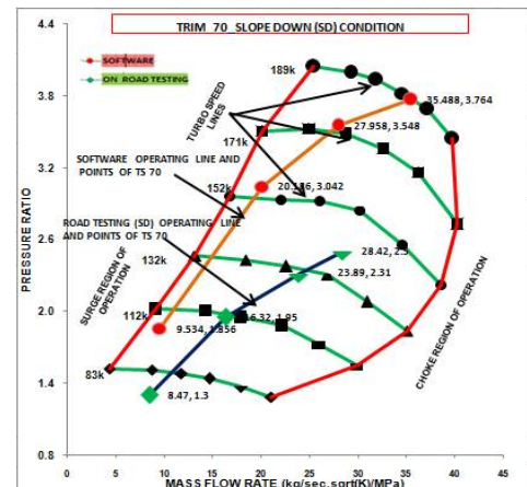
Fig. 11 Turbo match - slope-down - A58N70
