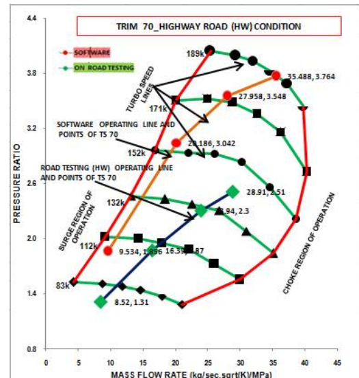
Fig. 5 Turbo match - Highway - A58N70
