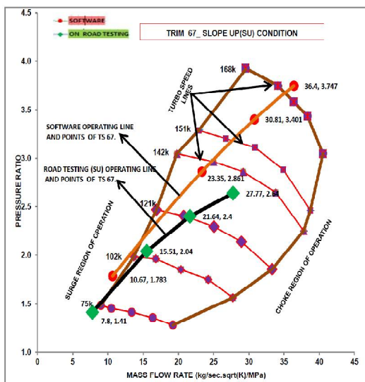
Fig. 8 Turbo match - slope-up -B60J67
