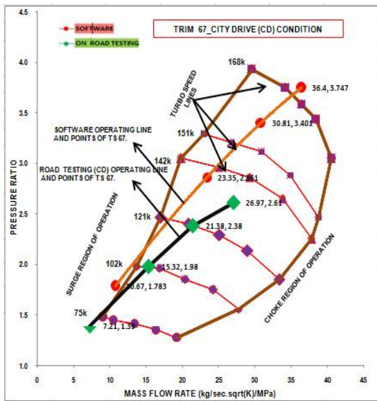
Fig. 6 Turbo match- City Drive - B60J67
