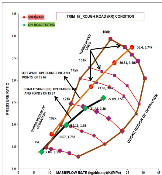
Figure2 Turbo match - Rough Road -B60J67
