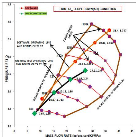
Fig.10 Turbo match – slope-down -B60J67
