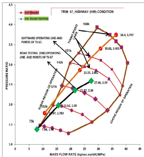
Fig. 4 Turbo match - Highway -B60J67
