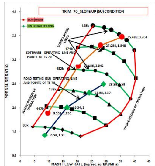
Fig. 9 Turbo match - slope-up - A58N70
