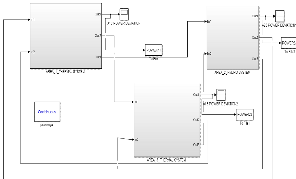
SIMULINK MODEL FOR SIMULATION OF LOAD FREQUENCY CONTROL USING GENETIC TUNING OF PID CONTROLLER
