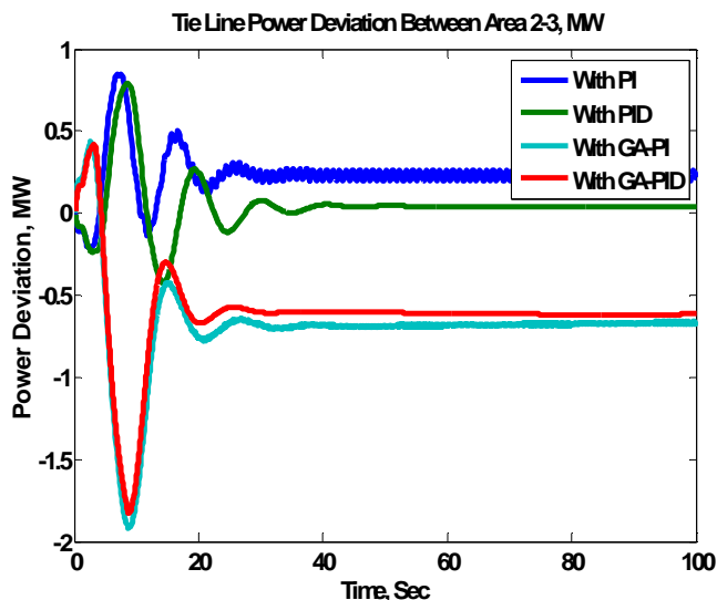
Fig.8 Tie Line Power Deviation Of Area 2-3
