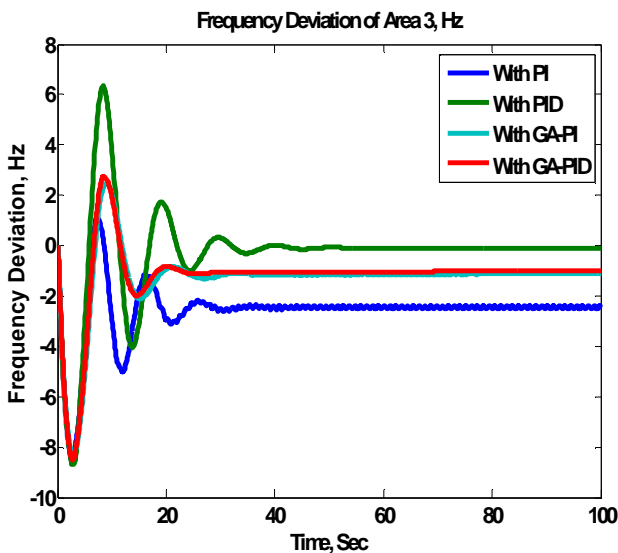
Fig.5 Frequency Deviation Of Area 3 Thermal System
