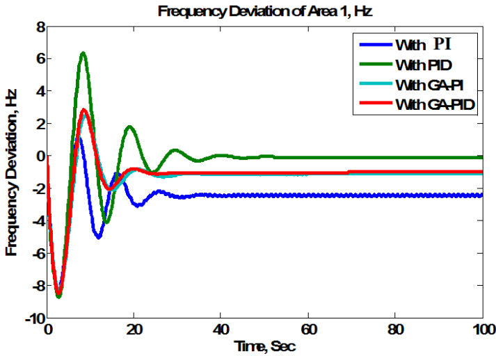
Fig.3 Frequency Deviation Of Area 1 Thermal System
