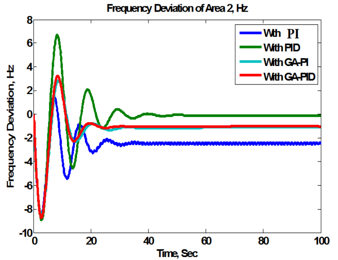
Fig.4 Frequency Deviation Of Area 2 Hydro System
