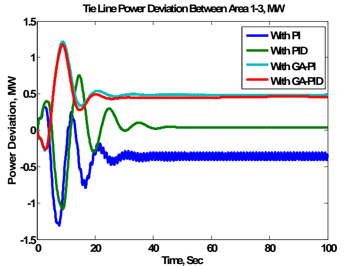
Fig.8 Tie Line Power Deviation Of Area 1-3
