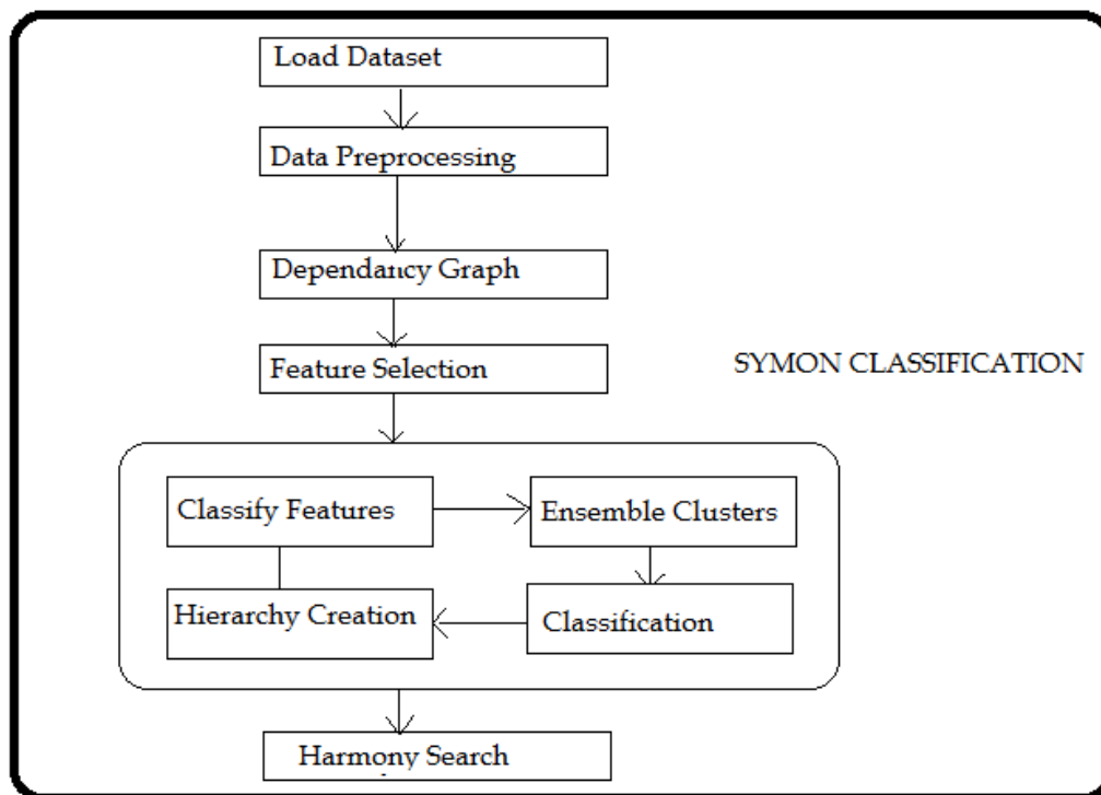
Fig. 1 System Architecture
