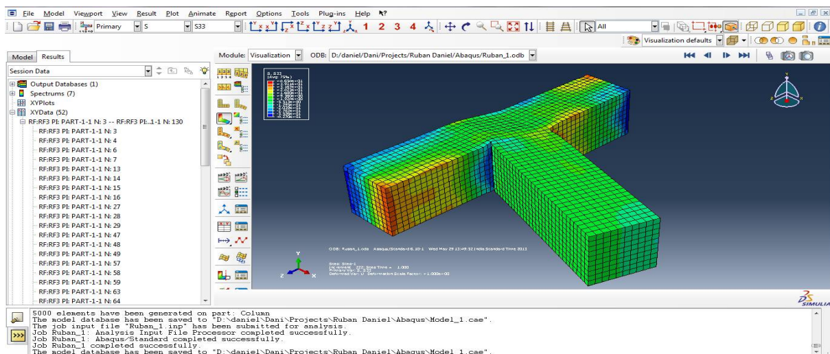
Stress contour of control specimen
