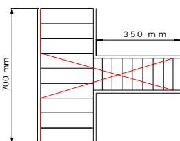
Fig 3 Indicates specimen having longitudinal beam bars with inclined anchorage.(BRACING 1)
