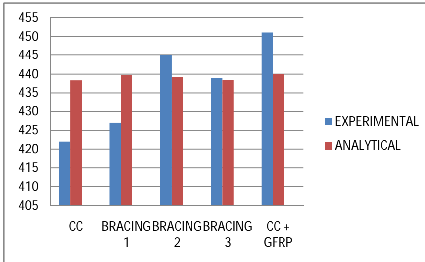
Comparison of Experimental and ABAQUS Load Carrying Capacity of Beam Column Specimens
