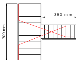
Fig 4 It had four inclined bars that extend from column to beam, two from the column portion above the joint and two from the column portion below the joint.(BRACING 2)
