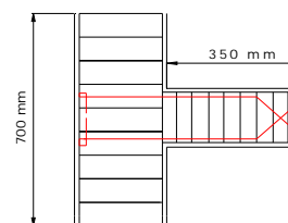
Fig 5 It provided with four supplementary bars in beam, two at top and two at bottom which were intersected to form 'X' shape.(BRACING 3)
