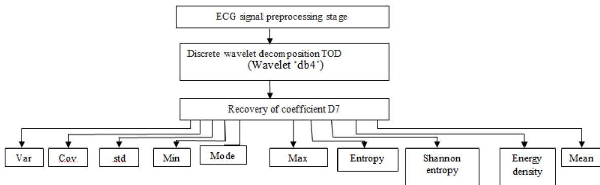
Fig 6: Principle of the algorithm for extracting statistical parameters
