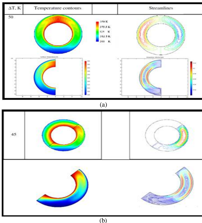
Figure 2 (a) Comparison between data of present work (lower line) and data of [5] (top line) for symmetric case and temperature difference of 50 °K.
