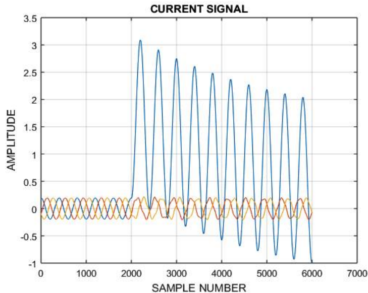
Figure No. 3 A-G type of Fault current signal
