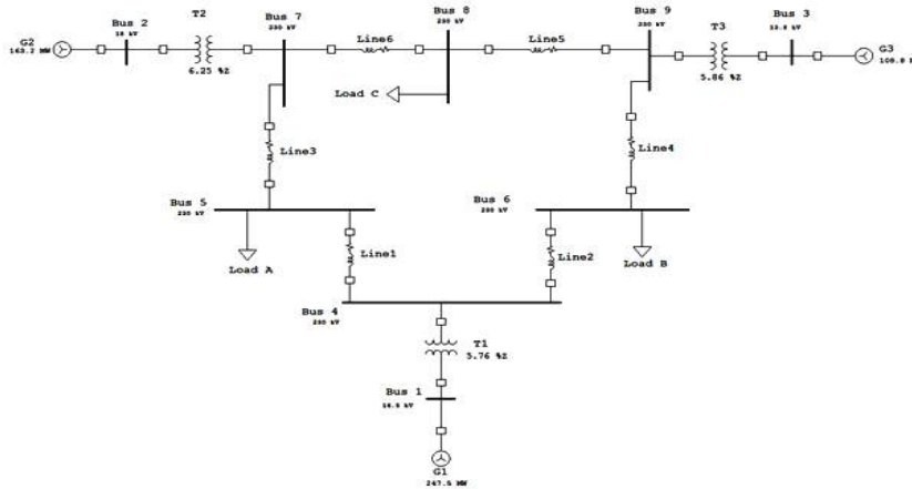
Figure No. 2 Single diagram of 3-machine 9-bus system.
