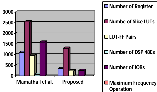
Figure 4: Bar Graph of the 8-point DCT
