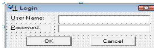
Fig 2. Login Screen
