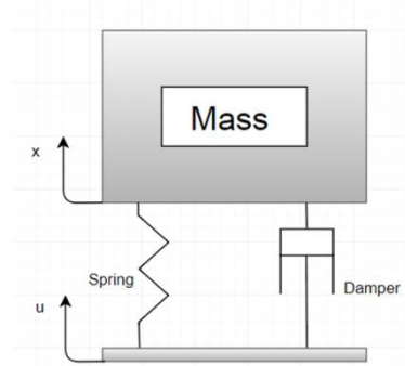
Fig 3: Active Suspension System.
