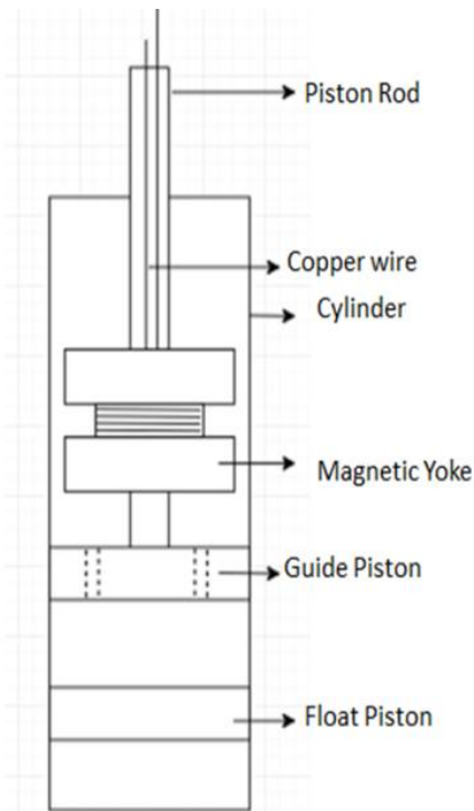
Fig 4: Schematic diagram of MR damper.
