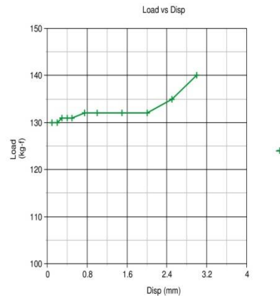
Fig 11: Force v/s Displacement graph at 1 Amp.
