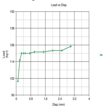
Fig 8: Force v/s Displacement graph at 0 Amp.
