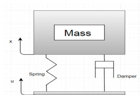
Fig 2: Passive suspension and semi-active suspension system
