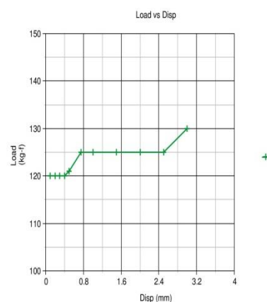
Fig 9: Force v/s Displacement graph at 0.5 Amp.
