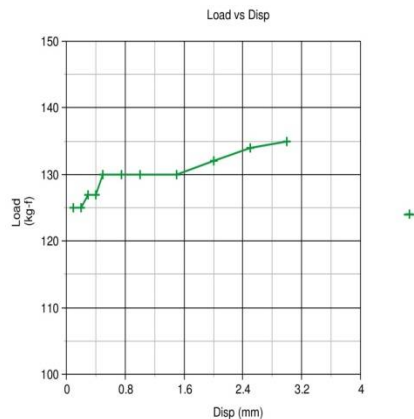
Fig 10: Force v/s Displacement graph at 0.8 Amp.
