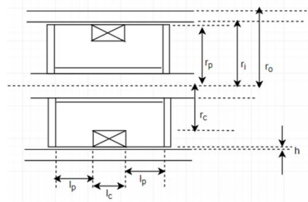
Fig 5: Design parameters of MR damper.
