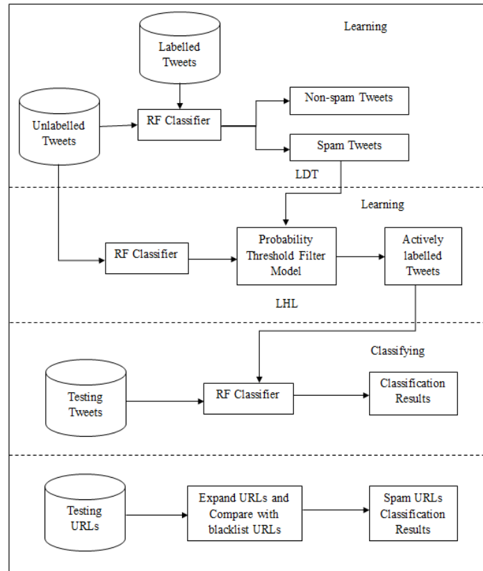
Fig.1 Lfun Framework
