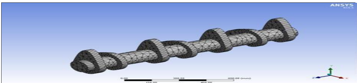
Fig.4. Meshed model
