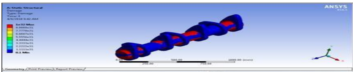
Fig.10. Damage of Camshaft
