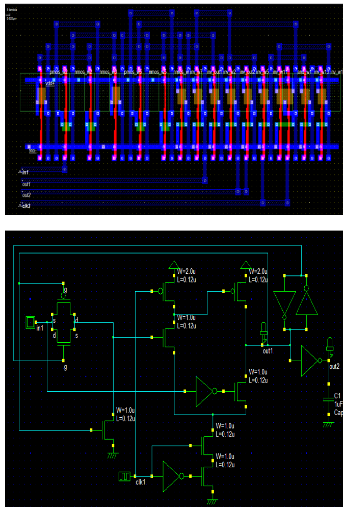
Figure 2: Schematic level for CPSFF.
