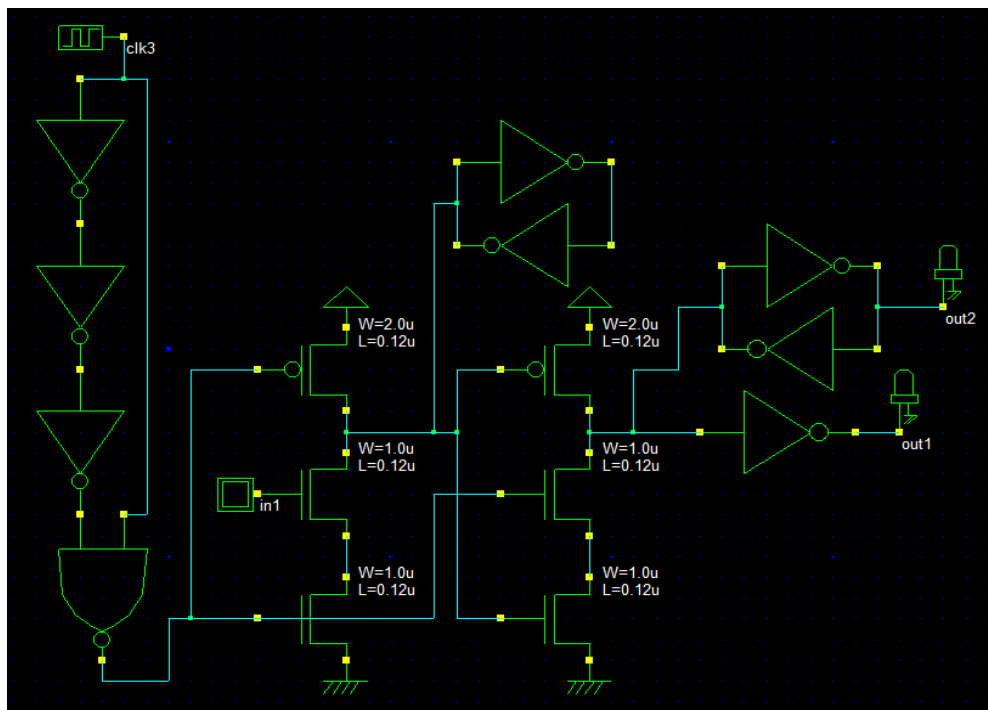
Figure 1: Schematic level for convention P-FF
