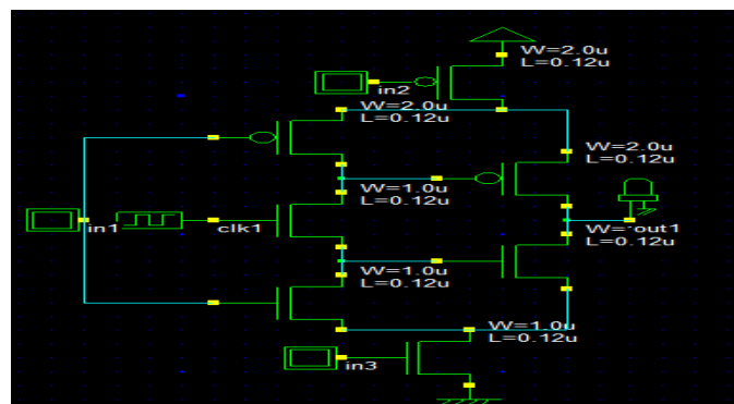
Figure 3: Schematic level for MTCOS.
