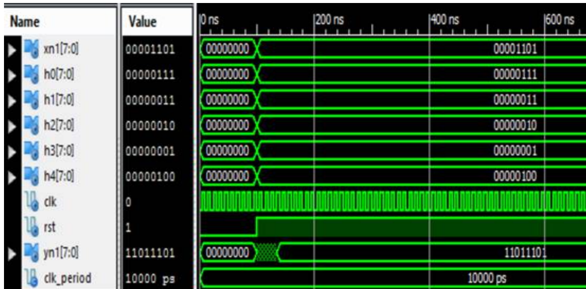
Fig. 5: Output Test Bench Waveform of Narrow Band Filter (Filter Coefficient N=5)
