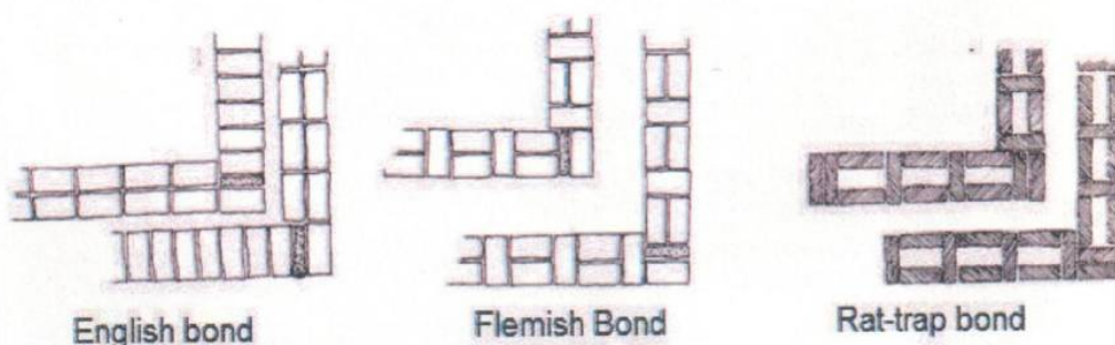
Figure2. Various Bonds in Brick Masonry
