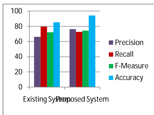
Fig. 4 Performance Analysis between existing and proposed system
