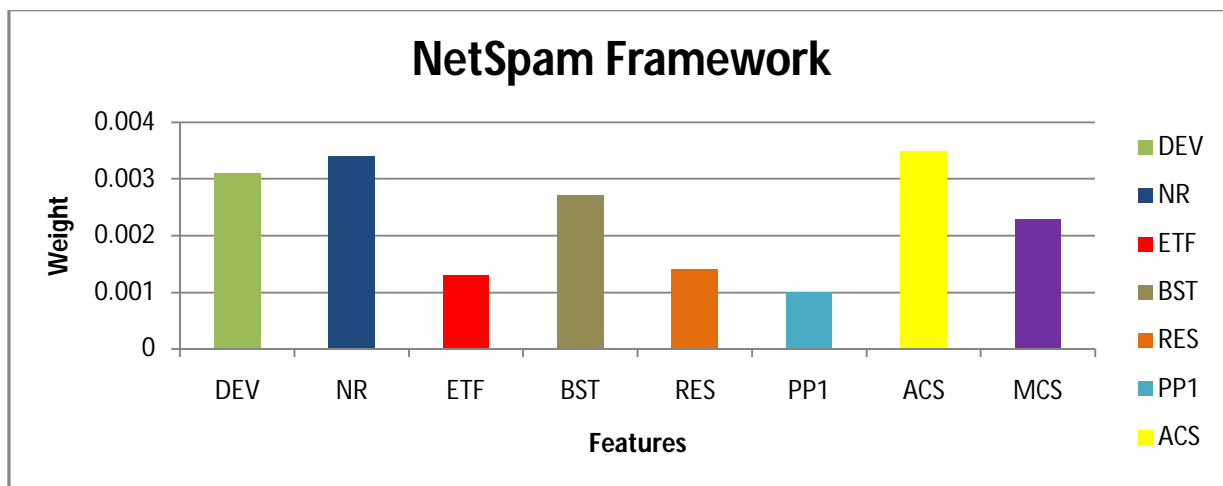
Fig.3 Feature weights for NetSpam Framework
