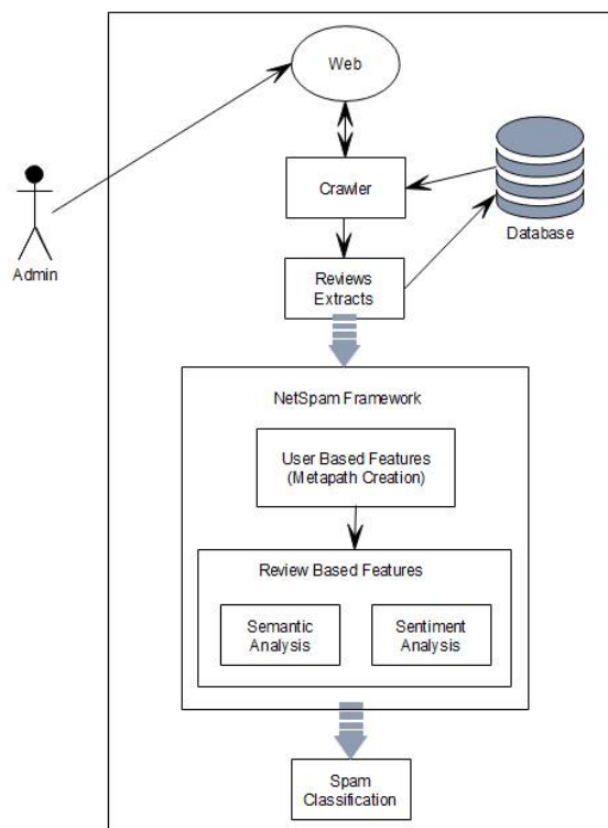
Fig No 01 System Architecture
