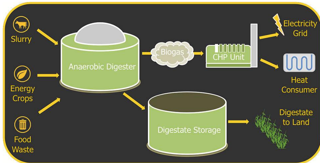
Figure 6: Anaerobic digestion
