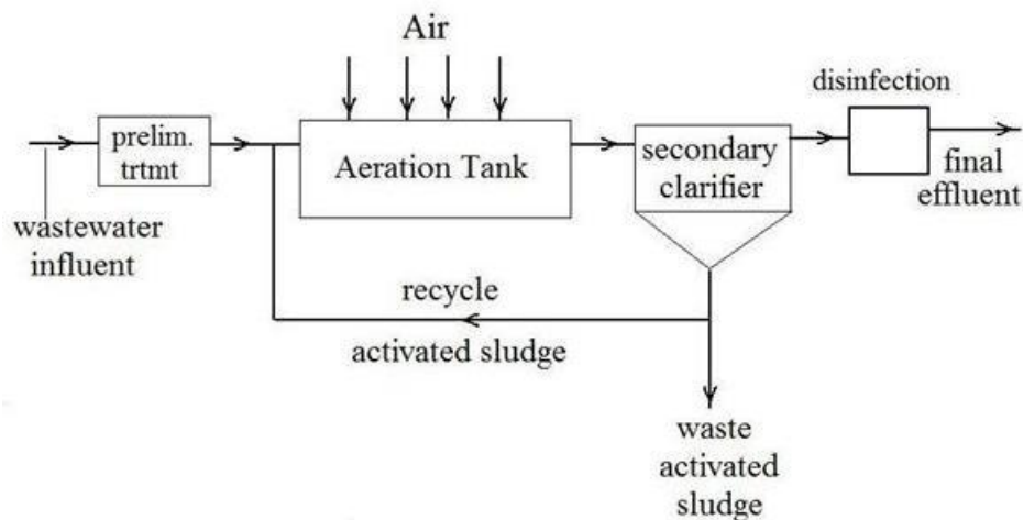
Figure 7: Activated Sludge Process (Flow diagram)
