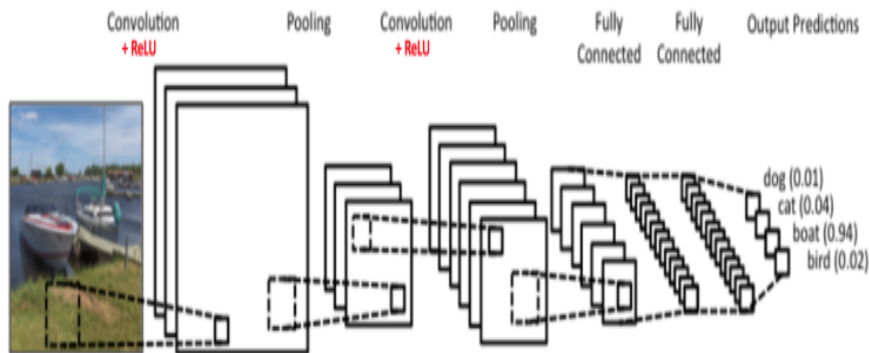
Fig2. Simple ConvNet
